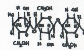
Cellulose structure
